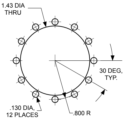
VIEW "A"
