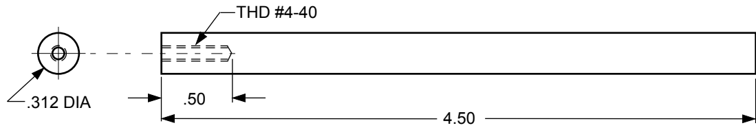
UPPER SUPPORT POST
