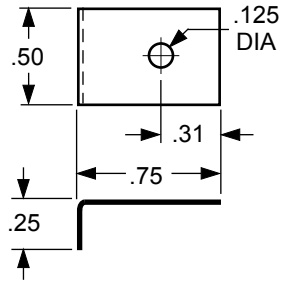
LOWER CLIP
