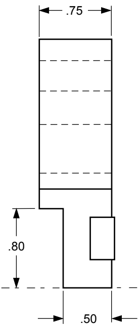
LOWER SUPPORT ASSEMBLY
